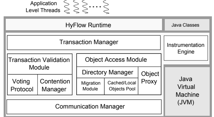
Figure 3. HyFlow Node Architecture
