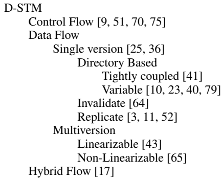
Figure 2. A distributed memory models taxonomy
