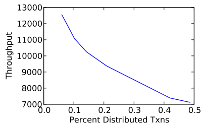
Figure 11: Total transactional throughput (3 warehouses), with a varying fraction of distributed txns.
